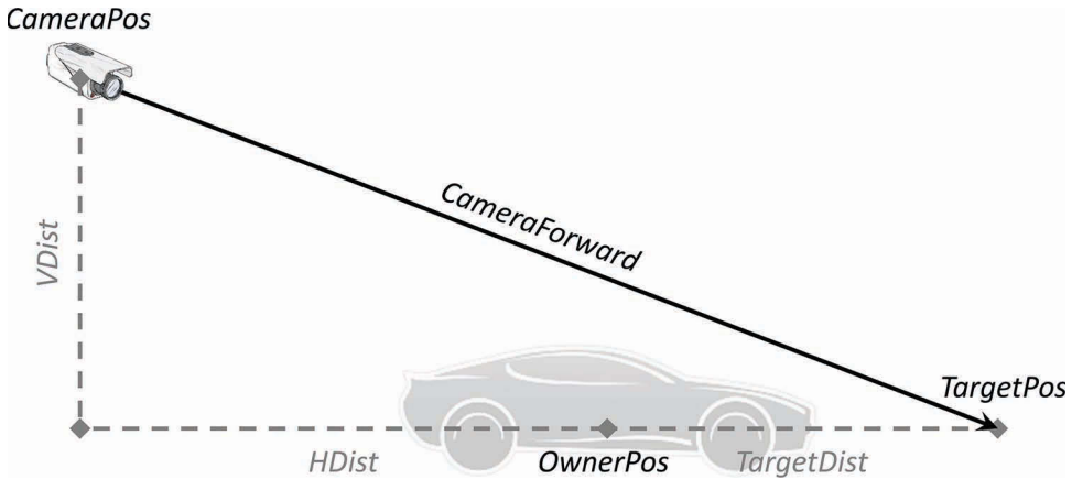
Figure 9.2 Basic follow camera tracking a car
