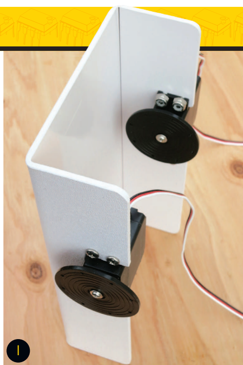
Figure I: Each servo is bolted into a notch cut in the frame. The wheels were included with the servo recommended for this project.
