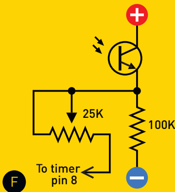
Figure F: A phototransistor can be substituted for each photoresistor, using a 100K resistor as shown here. Servo control may be rougher. Make sure the shorter lead connects with the positive power supply.
