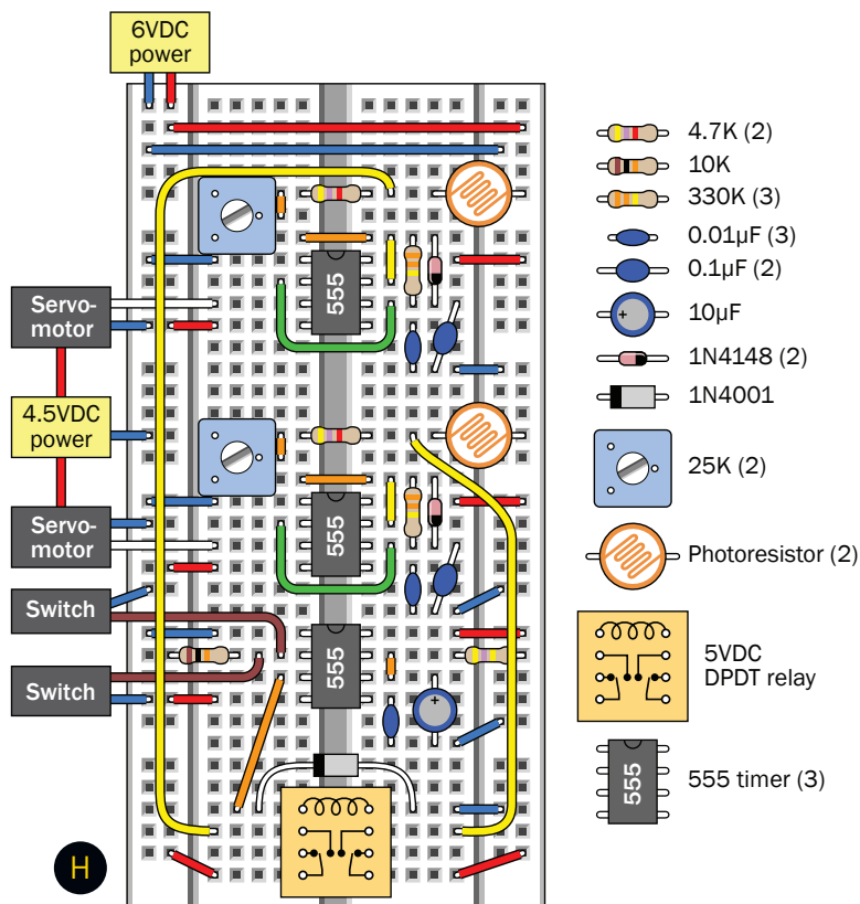
Figure G: The complete schematic for control electronics to run your obedient servo.
